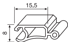
55 5605 Profile Length : 2500mm
