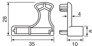
30 3620/01 Left Right End Cap (For 55 5981)
