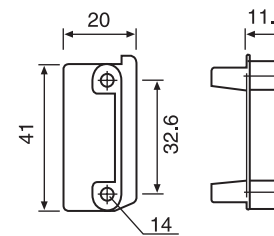
Left Right End Cap (For 55 6098) 303722/3
