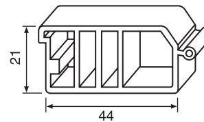
55 6098 Lock Section Profile Length : 2500mm
