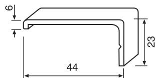
50 5895 Fascia Profile Length : 2500mm
