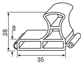
55 5981 Handle Profile Length : 2500mm
